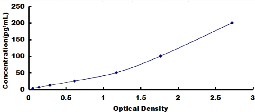
Typical Standard Curve of ELISA Assay for Gallus, IFN \beta .
