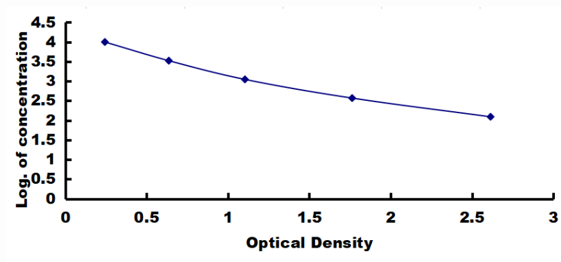
Typical Standard Curve of ELISA Assay for PCr.
