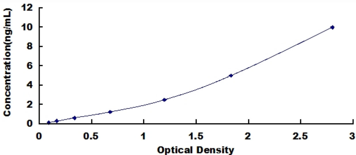
Typical Standard Curve for C5a, Rat ELISA.
