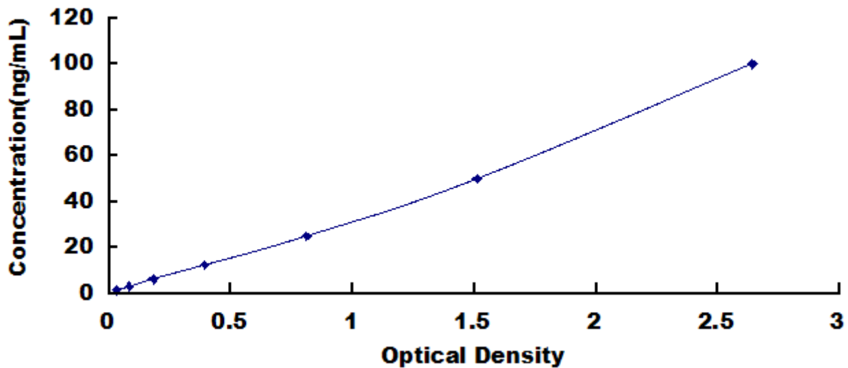
Typical Standard Curve for EPCR, Mouse ELISA.
