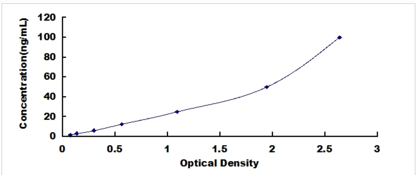
Typical Standard Curve for Myeloperoxidase, Bovine ELISA.
