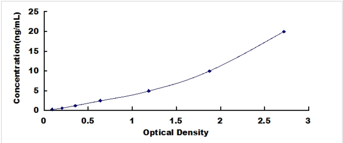
Typical Standard Curve for PRMT1, Human ELISA.
