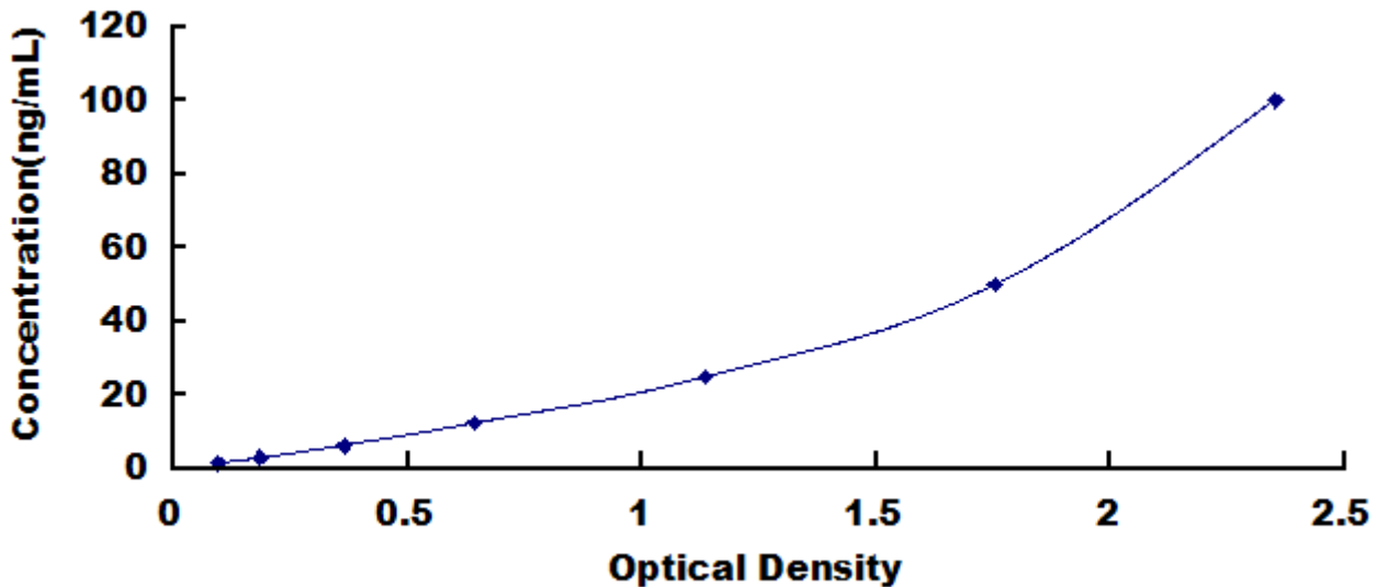
Typical Standard Curve for PDHa, Human ELISA.
