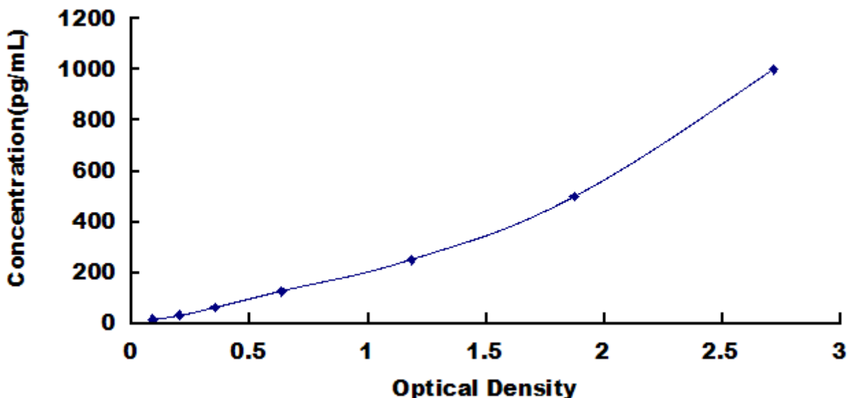
Typical Standard Curve for COL1, Human ELISA.
