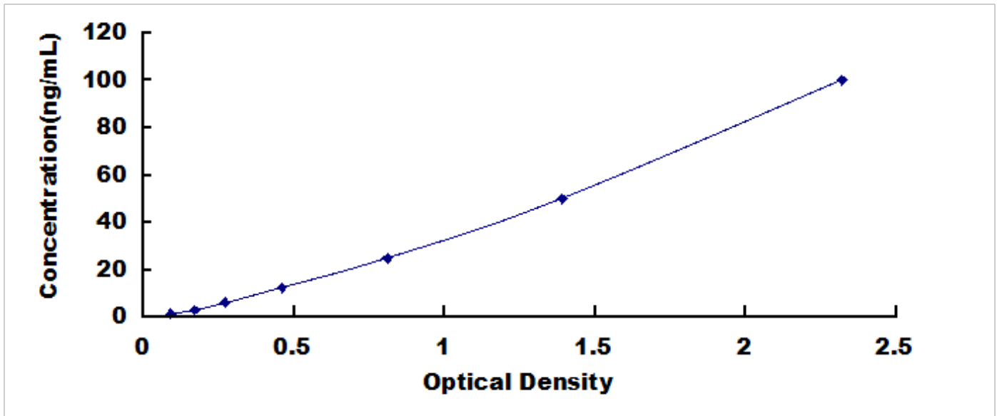
Typical Standard Curve for CYPA, Mouse ELISA.
