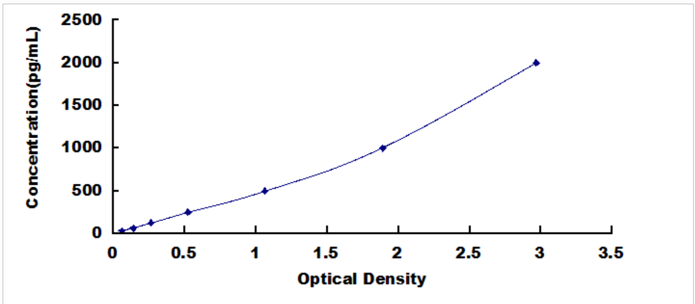
Typical Standard Curve for cTnI, Rat ELISA.
