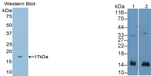
Figure. Western Blot; Sample: Recombinant IFN \gamma , Mouse.
